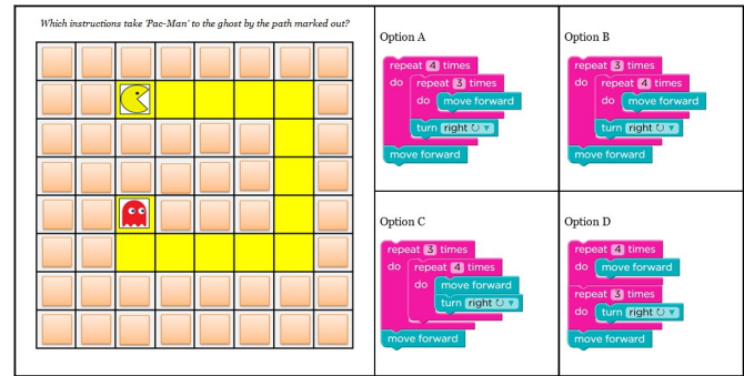
Figure 1: CT Test, item #8 ('maze'): loops 'repeat times' (nested); 'visual blocks'; 'sequencing'.
